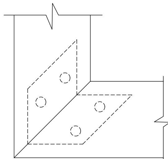
CORNER DETAIL WITH CORNER CLIP WELDED IN
