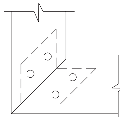
CORNER DETAIL WITH CORNER CLIP WELDED IN
